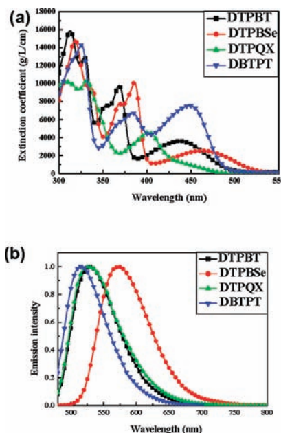
Figure 3. Absorption spectra (a) and emission spectra (b) of all the fused D-A molecules in toluene.
